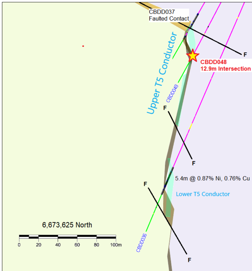
Figure 6: Cross Section showing drill intercept and their relationship to the T5 conductor.
