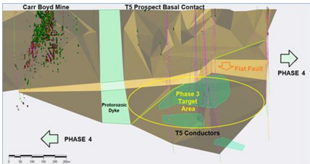
Figure 5: Locations that are to be targeted in Phase 3. The flat fault has a lateral throw of 80m to the East.
