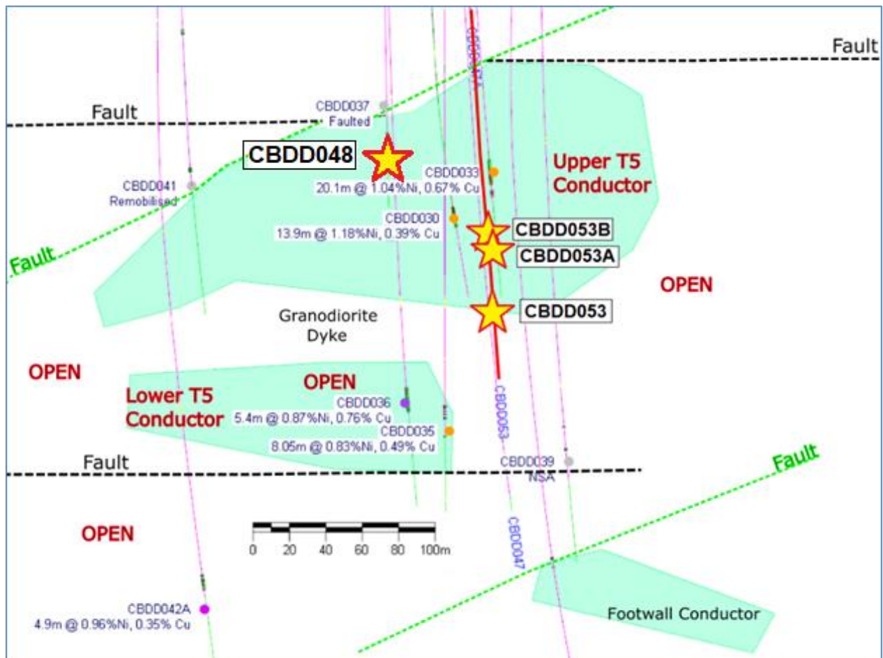
Figure 4: Longsection showing the CBDD048 intersection in relation to other significant intersections and the T5 downhole electromagnetic (DHEM) Conductors.
